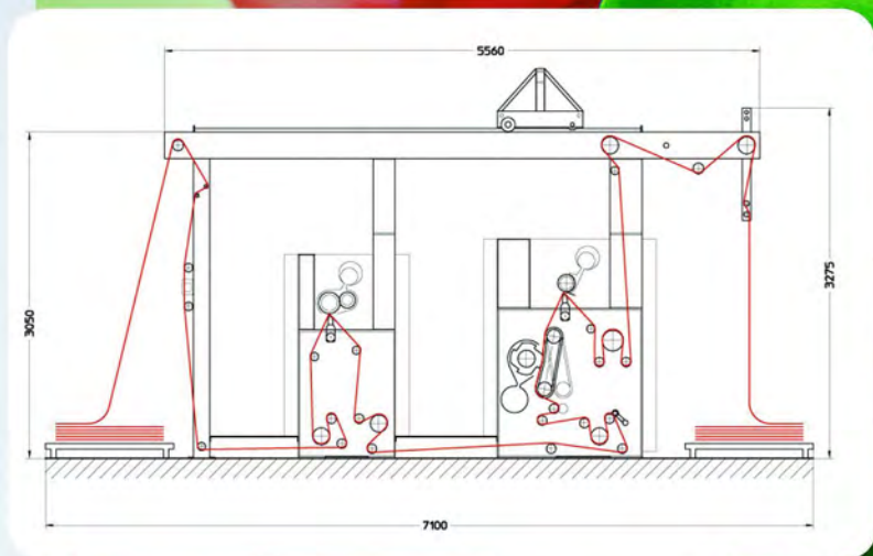
Tri-combined Tigering, Polishing and Shearing machine.
