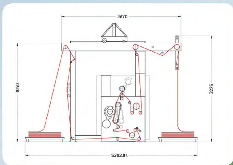
Combined Polishing and Shearing machine.
